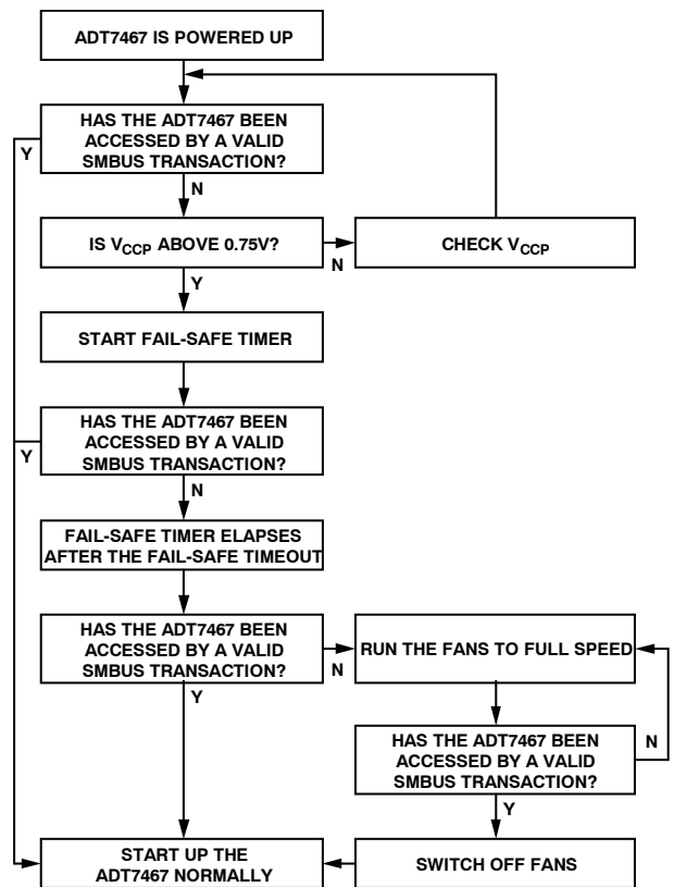
Figure 48. Power-On Flowchart
